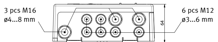
Wall-mounted MULTICAL® 801 seen from the side MULTICAL® 801 cable connections
