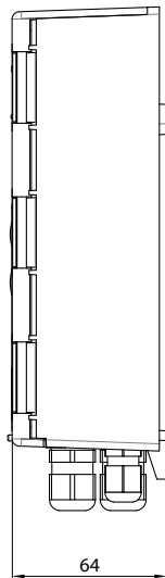
Wall-mounted MULTICAL® 801 seen from the side MULTICAL® 801 cable connections
